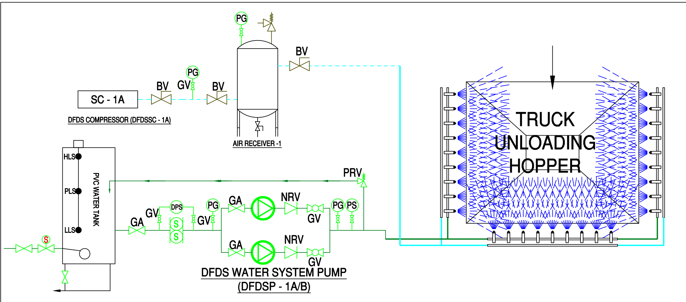
DRY FOG DUST SUPPRESSION SYSTEM FOR TRUCK UNLOADING HOPPER
